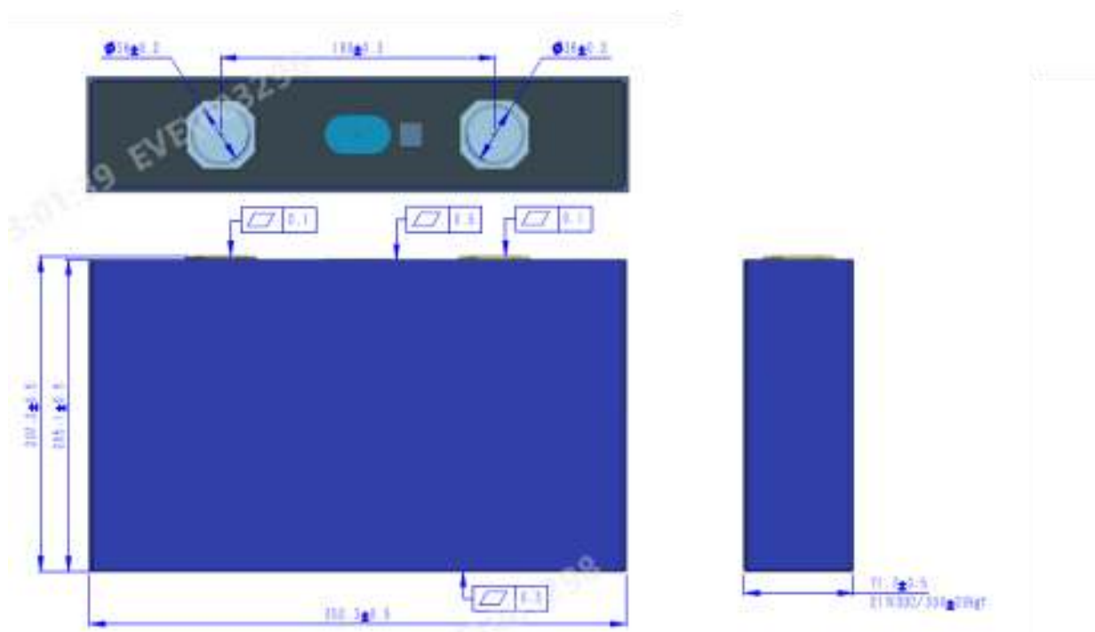
Fig. 15 Diagram of cell size and appearance 图 15 电池尺寸及外观图
